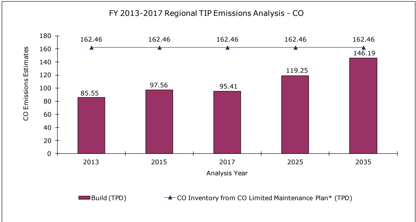
Figure 7: Comparison of the CO “Build” Scenario to the CO and PM 10 Inventories
