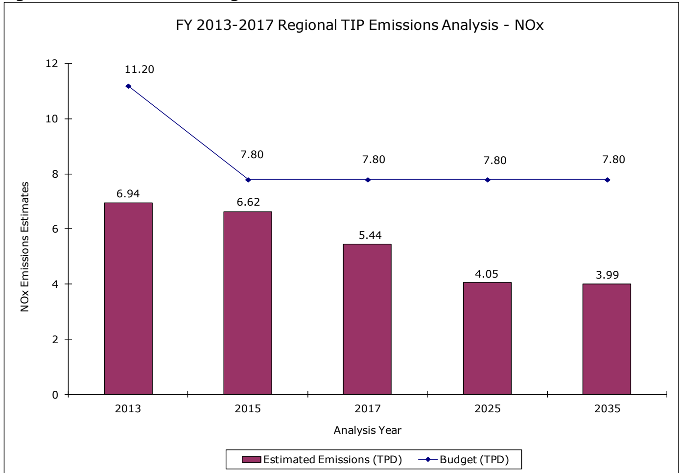
Figure 4: Results of NO x Budget Test
