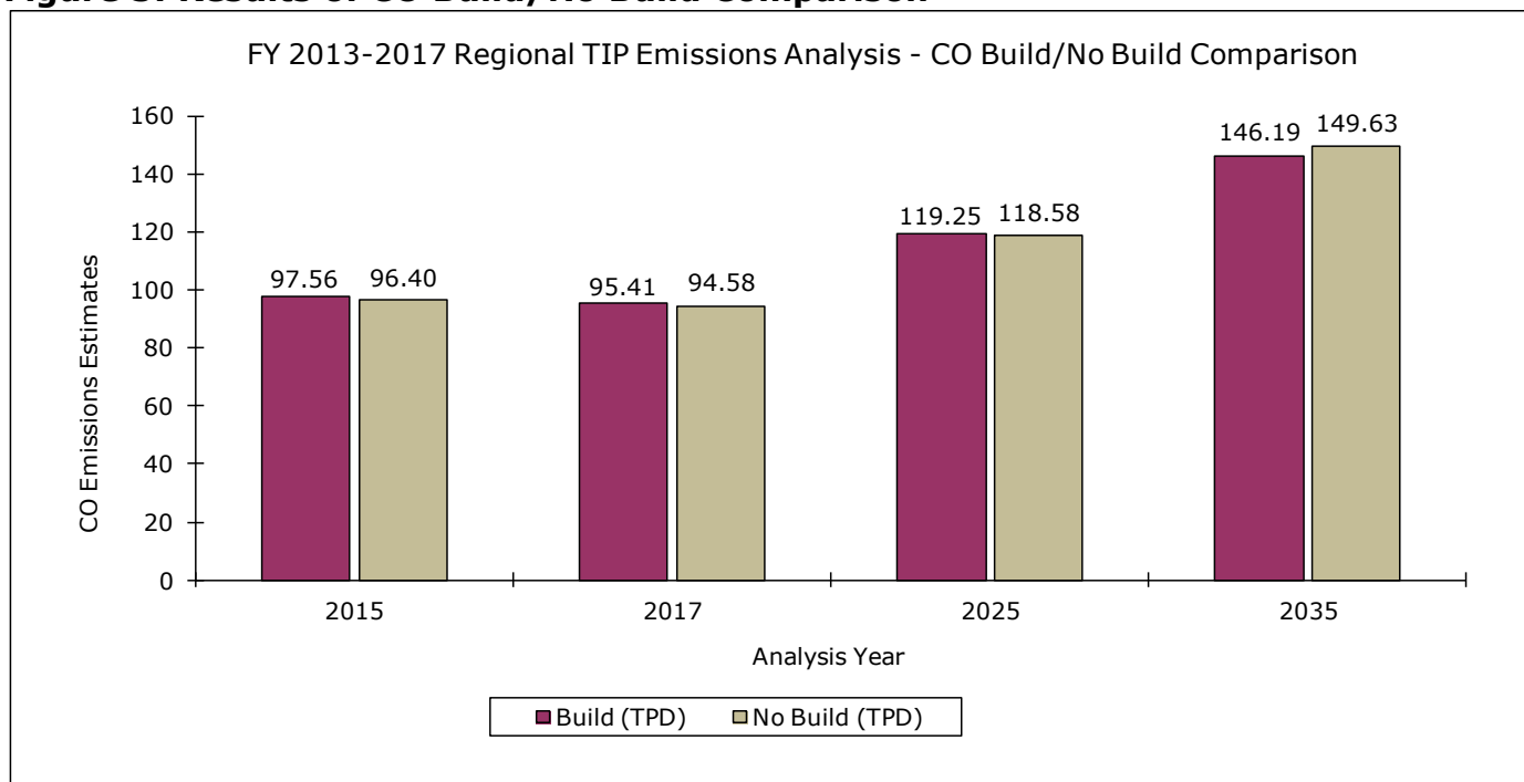
Figure 5: Results of CO Build/No Build Comparison
