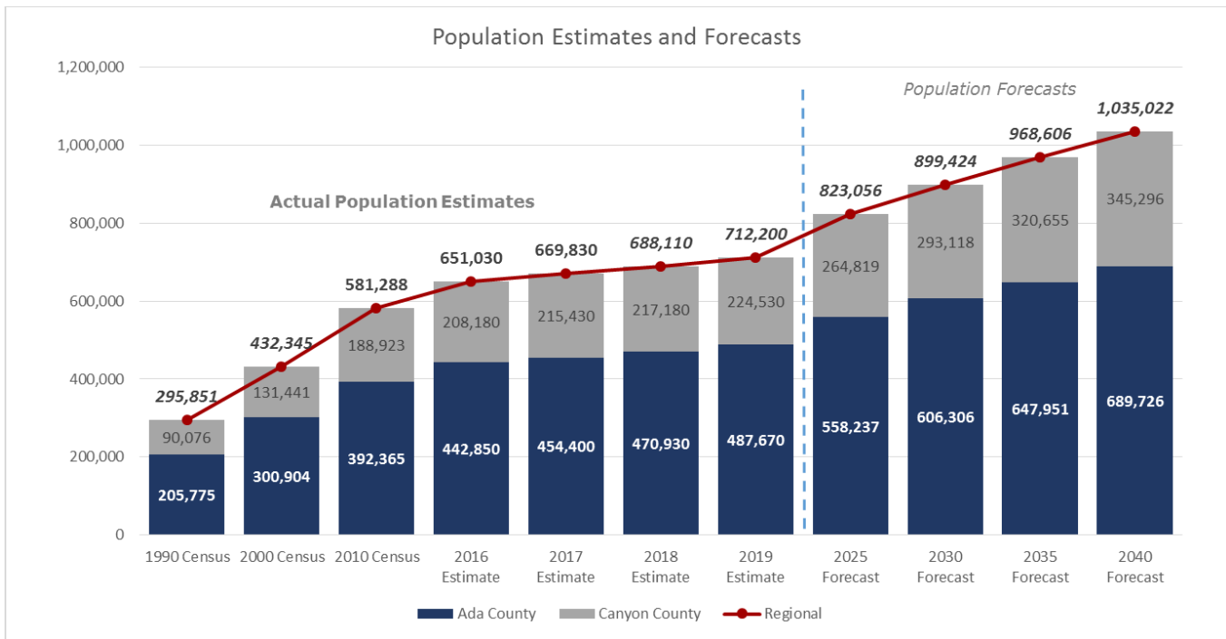
Figure 1: COMPASS Population Estimates 14 and Forecasts
