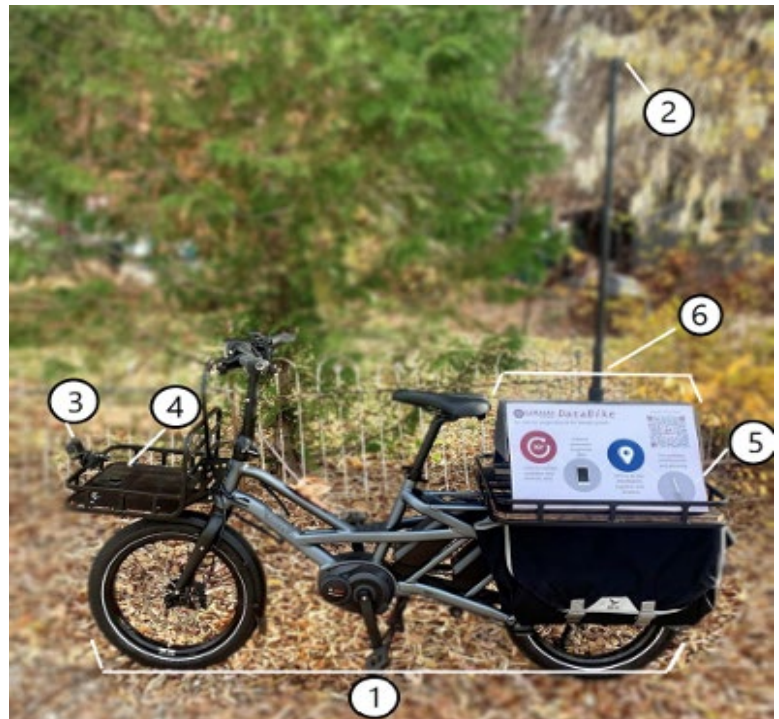
Figure 3: COMPASS Data Bike with Data Collection Equipment
